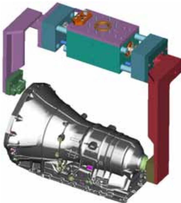
Large Part Gripper
